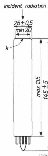
Dimensions (in mm) and electrode connections
