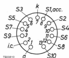
13-pins socket type No. B8 700 67
