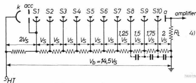
Voltage divider type B
