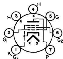
BASING DIAGRAM JEDEC 7CV BOTTOM VIEW
