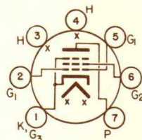
BASING DIAGRAM JEDEC 7CV BOTTOM VIEW
