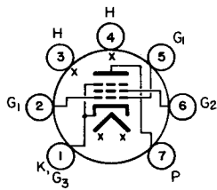
BOTTOM VIEW BASING DIAGRAM JEDEC 7CV
