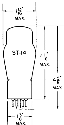
GLASS BULB
