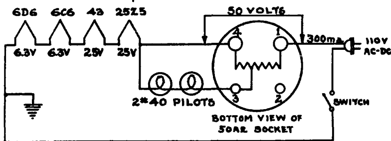
• TYPICAL FILAMENT & PILOT CIRCUIT FOR AC-DC RADIOS •
