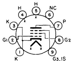
BOTTOM VIEW BASING DIAGRAM JEDEC 9 PM
