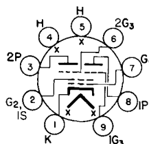
BOTTOM VIEW BASING DIAGRAM JEDEC 9FG
