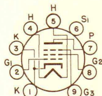
BASING DIAGRAM
