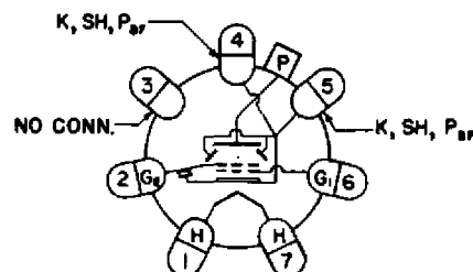
BOTTOM VIEW OF SOCKET TYPE RK-4D32
