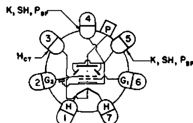
BOTTOM VIEW OF SOCKET TYPE RK-4D22
