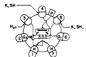
BOTTOM VIEW OF SOCKET TYPE RK-4D22
