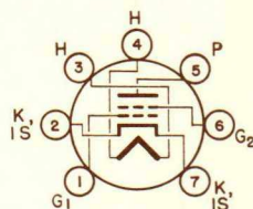
BOTTOM VIEW BASING DIAGRAM JEDEC 7EW
