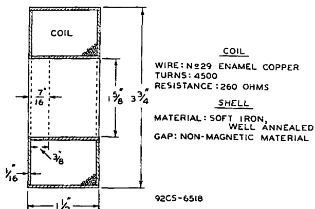
Fig. 3 - Focusing-Coil Details.
