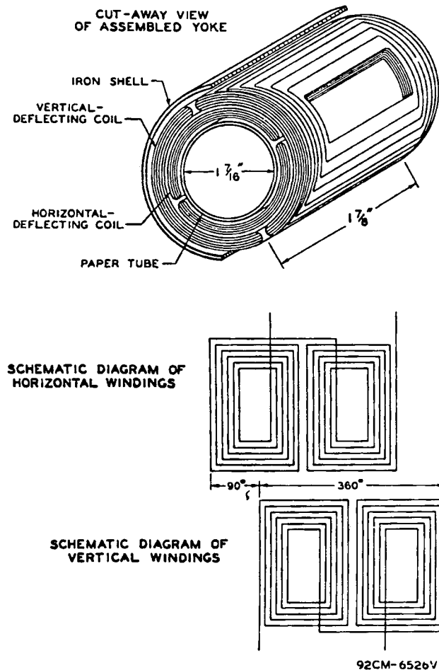
Fig. 1 - Wide-Angle Deflecting Yoke Assembly and Winding Scheme.
