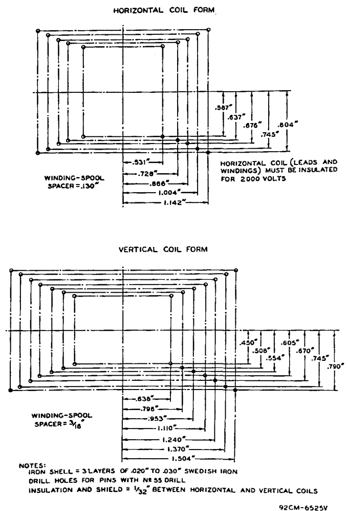
Fig. 2 - Coil Form Details of Wide-Angle Deflecting Yoke.
