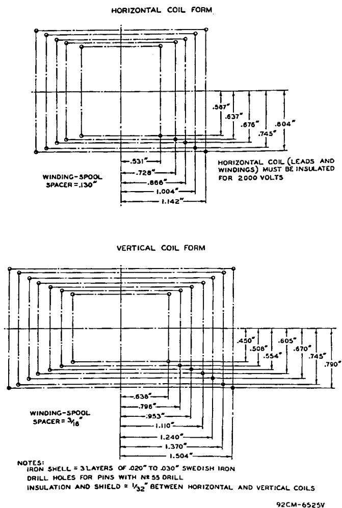
Fig. 2 - Coil Form Details of Wide-Angle Deflecting Yoke.
