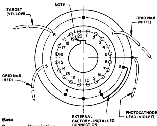
Enlarged Bottom View, Types 4807/V1 And 4807A/V1
