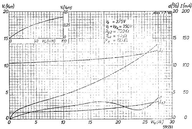
Fig. 7 Total distortion, anode and screen-grid current and alternating input voltage as functions of the output power; 2 valves 4699 used in class AB output stage with auto. grid bias, V_b = 375 V
