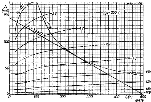
Fig. 4 Anode current as a function of the anode voltage for various values of grid bias with V_{g2} = 250 V.
