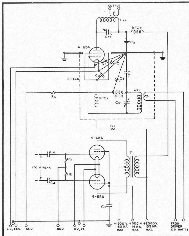
Typical high-level-modulated R-F amplifier, 240 watts plate input. Modulator requires zero driving power.
