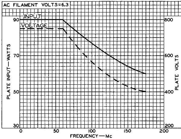
Fig. 4 - Maximum Ratings vs. Operating Frequency for Type 4604 in ICAS Class C Telegraphy or Telephony Service.
