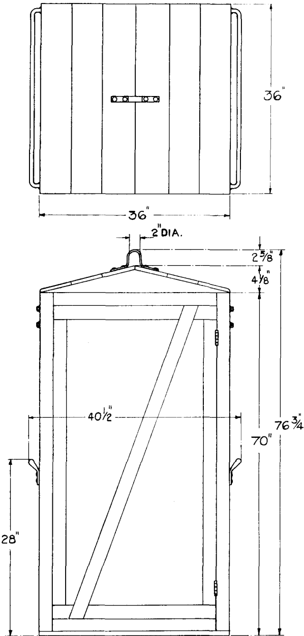
PACKING CRATE.
