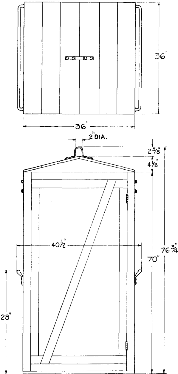
PACKING CRATE.
