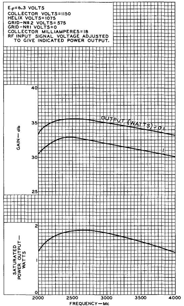
Fig.4 - Typical Characteristics of Type 4010.
