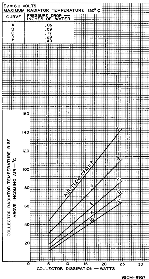
Fig. 1 - Cooling Requirements of Type 4010.
