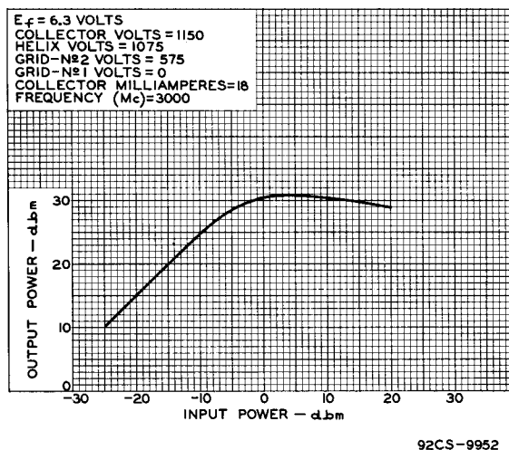
Fig. 3 - Typical Power Output Characteristic of Type 4010.
