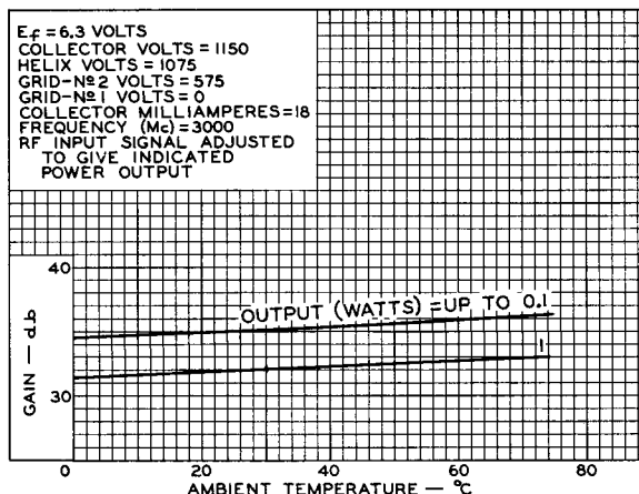
Fig. 2 - Typical Gain Characteristics of Type 4010.
