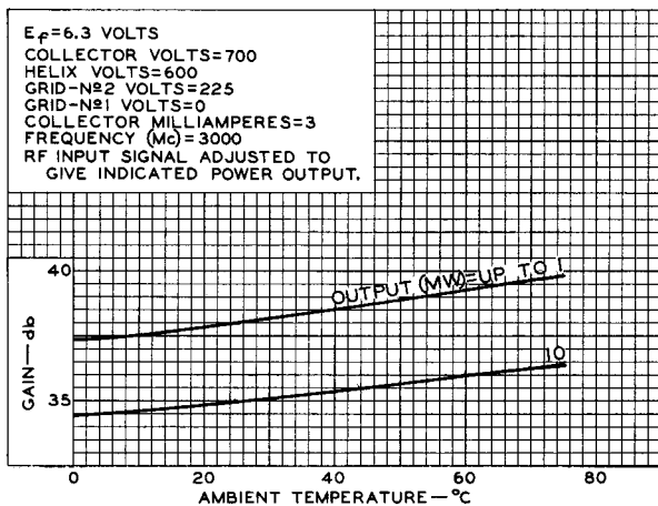
Fig. 1 - Typical Gain Characteristics of Type 4009.
