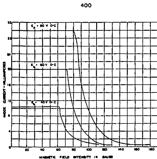
Typical Magnetic Control Characteristics K-8639678 8-29-44
