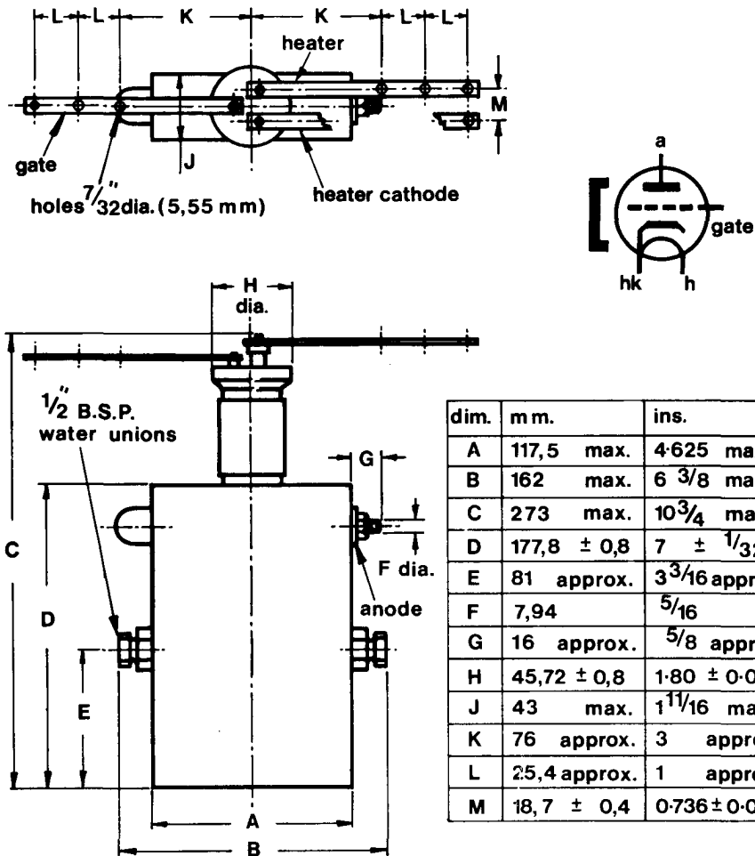
Fig. 4. Tube Outline
