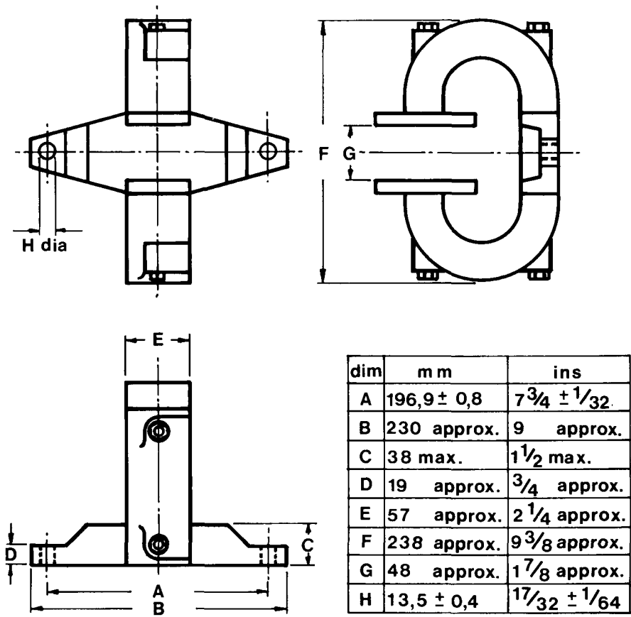
Fig. 5. Magnet Outline
