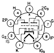
BOTTOM VIEW BASING DIAGRAM JEDEC 9FG
