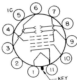
11N BOTTOM VIEW OF BASE
