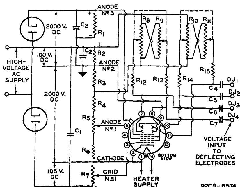
Typical Oscillograph Circuit
