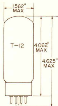
GLASS BULB SHORT MEDIUM-SHELL 5 PIN OCTAL B8-110 OR B8-118 OUTLINE DRAWING JEDEC 12-26
