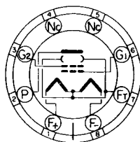
BOTTOM VIEW LOCK-IN 8 PIN BASE 688
