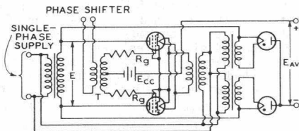
FIG. 3 SERIES SINGLE-PHASE
