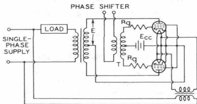
FIG. 4 FULL-WAVE SINGLE-PHASE
