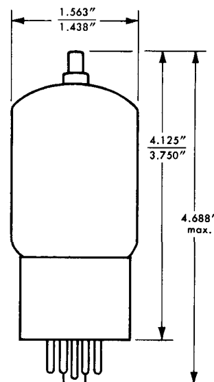
OUTLINE DRAWING
