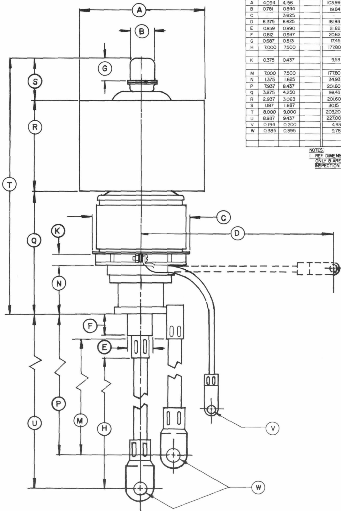
DIMENSIONAL DATA
