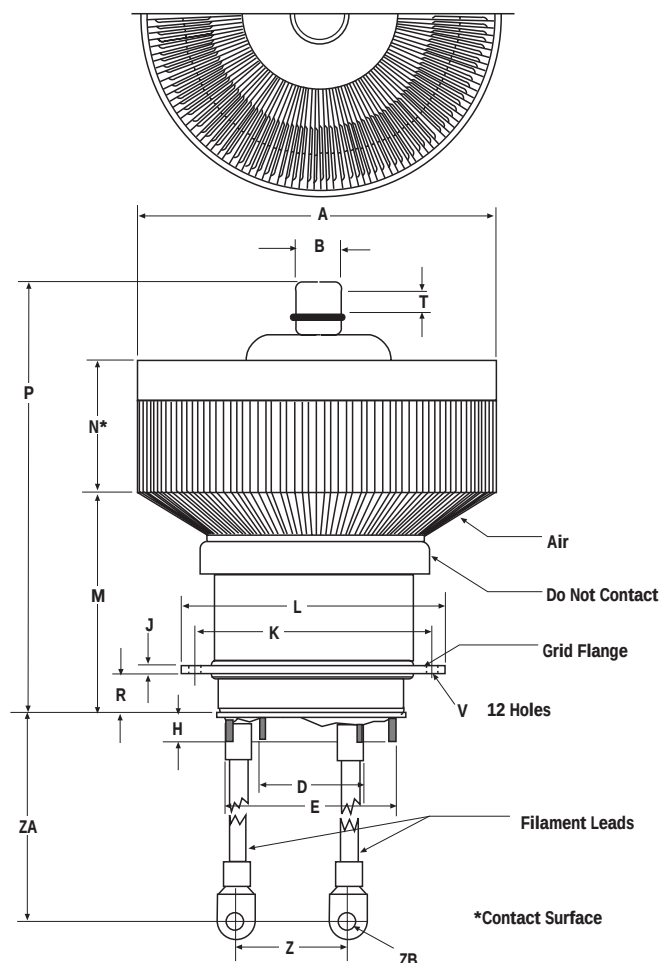
Svetlana 3CX15,000H3 Industrial Triode Outline Drawing
