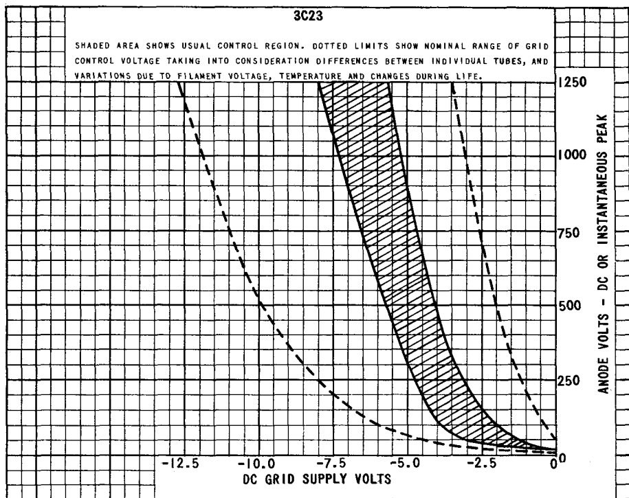
OPERATIONAL RANGE OF CRITICAL GRID VOLTAGE
