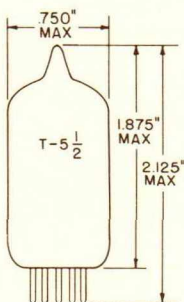
GLASS BULB MINIATURE BUTTON 7 PIN BASE E7-1 OUTLINE DRAWING JEDEC 5-7
