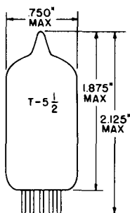
GLASS BULB MINIATURE BUTTON 7 PIN BASE E7-1 OUTLINE DRAWING JEDEC 5-9
