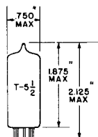
GLA-55 BULB MINIATURE BUTTON 7 PIN BASE E7-7 OUTLINE DRAWING JEDEC 5-2
