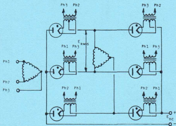
FIGURE 6 - FULL WAVE - THREE PHASE
