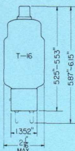
GLASS BULB
