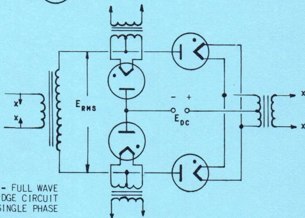
FIGURE 2 - FULL WAVE - SINGLE PHASE
