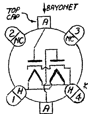
BOTTOM VIEW OF SOCKET
