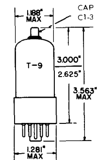
GLASS BULB INTERMEDIATE SHELL 6 PIN OCTAL B6-8 OR SHORT INTERMEDIATE SHELL 6 PIN OCTAL WITH BARRIERS B6-40
