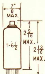
GLASS BULB SKIRTED MINIATURE CAP
