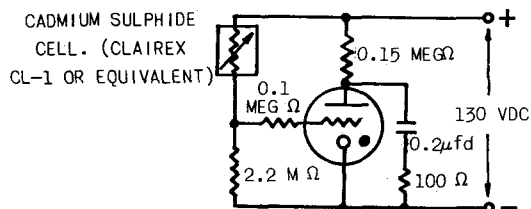
7400 ACTING AS A RELAY FOR A CADMIUM SULPHIDE PHOTO CELL
