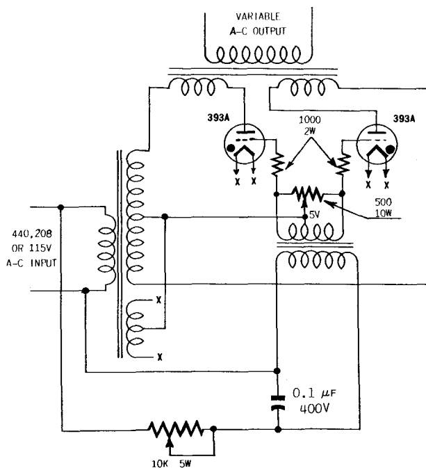
FIG. 3 THYRATRON POWER SUPPLY PROVIDING VARIABLE A-C OUTPUT FROM A-C INPUT
