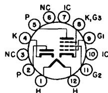
BOTTOM VIEW BASING DIAGRAM JEDEC 12 FS
