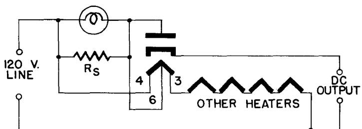
CIRCUIT 2
