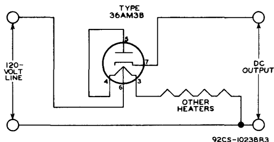
TYPICAL HALF-WAVE CIRCUIT
