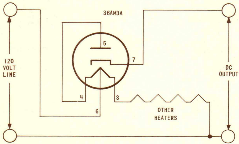
TYPICAL HALF-WAVE CIRCUIT
