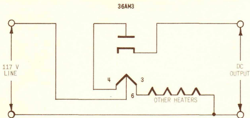
TYPICAL APPLICATION
