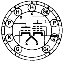
BOTTOM VIEW MINIATURE BUTTON 9 PIN BASE 9ME
