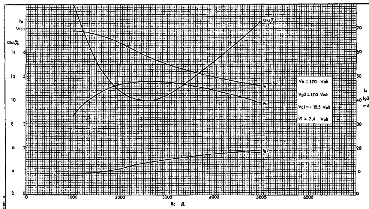
Fig. 6 — Average Characteristics
