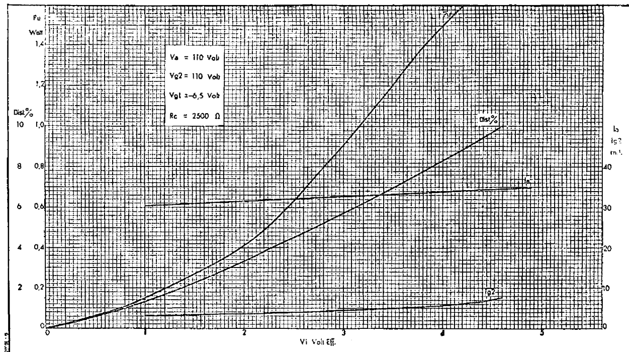
Fig. 3 — Average Characteristics
