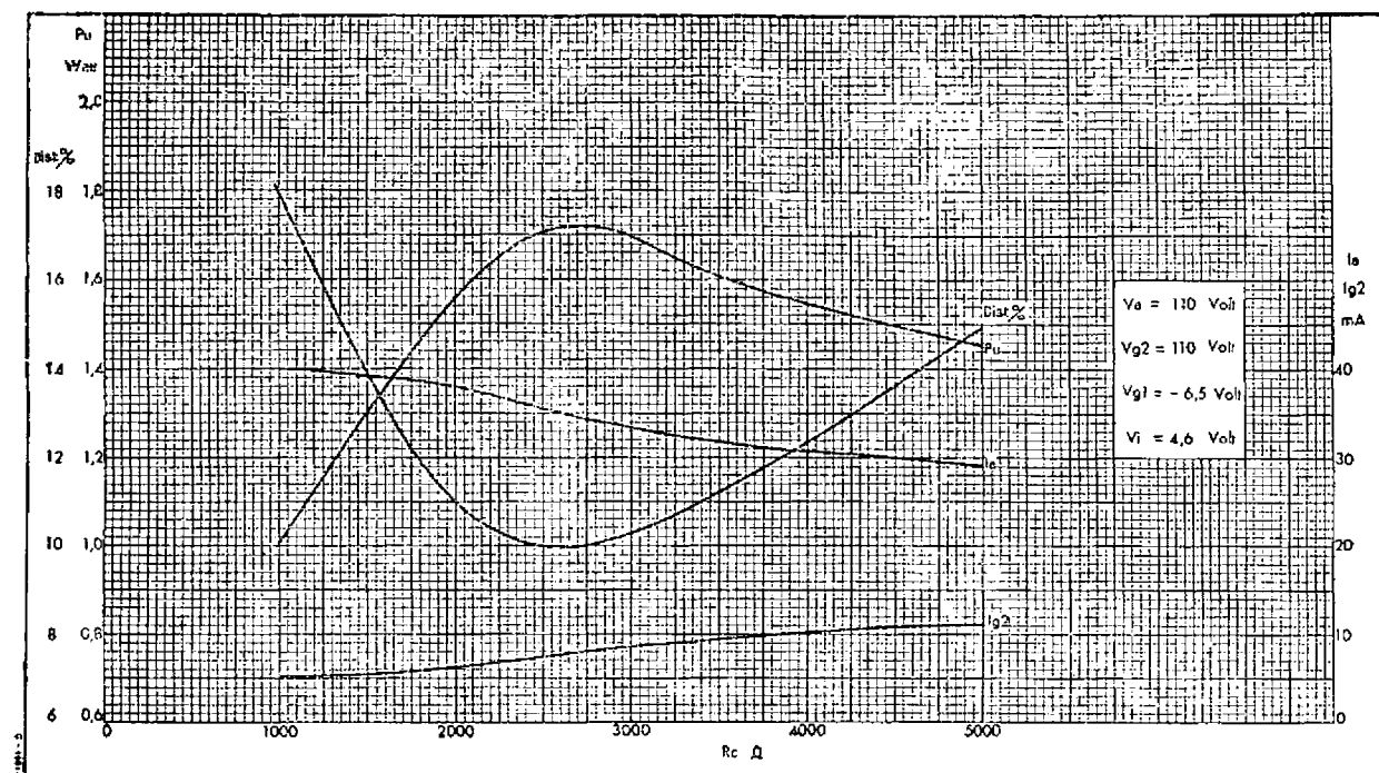
Fig. 4 — Average Characteristics
